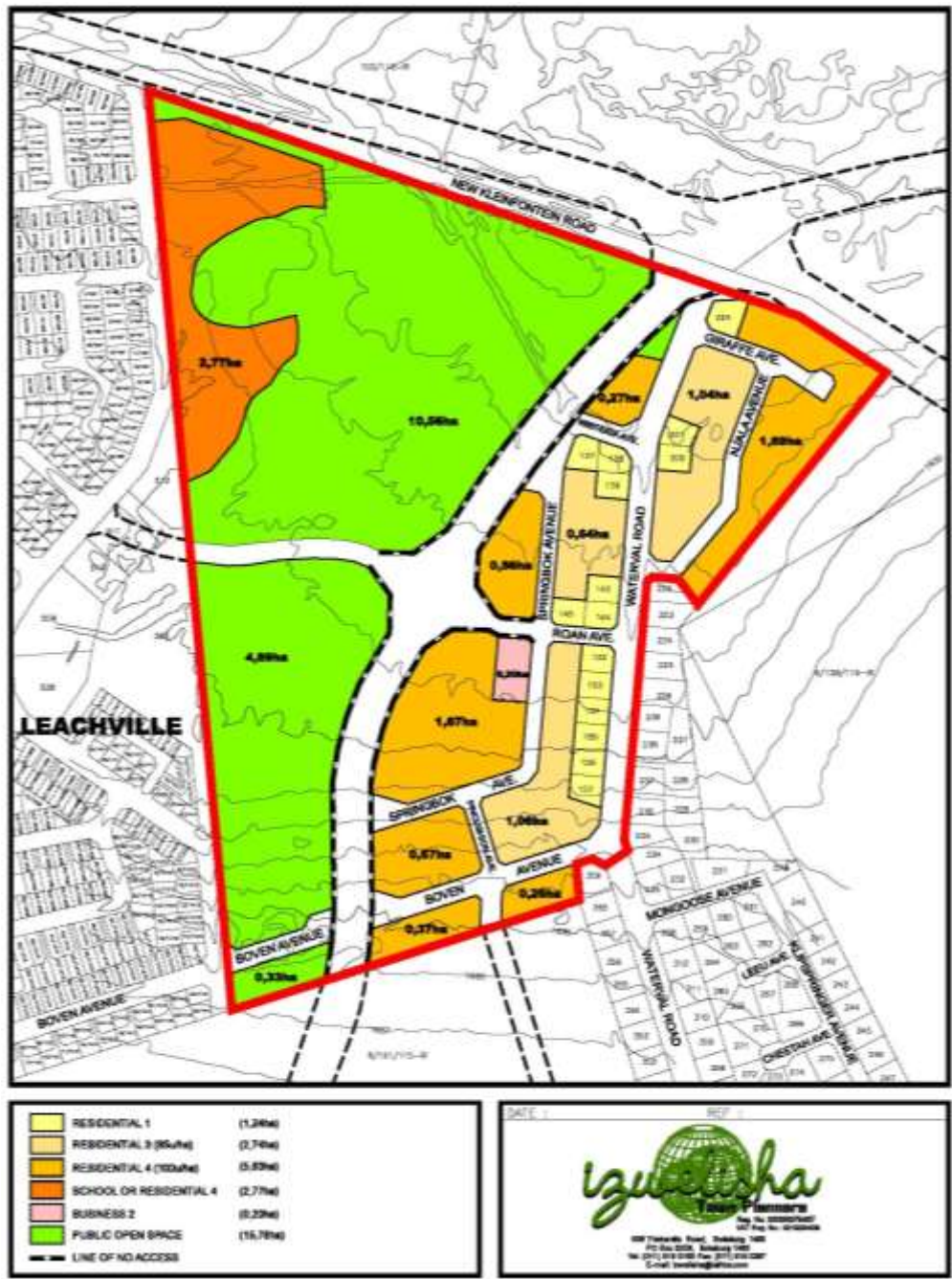
Figure 1: Site layout plan of the development
